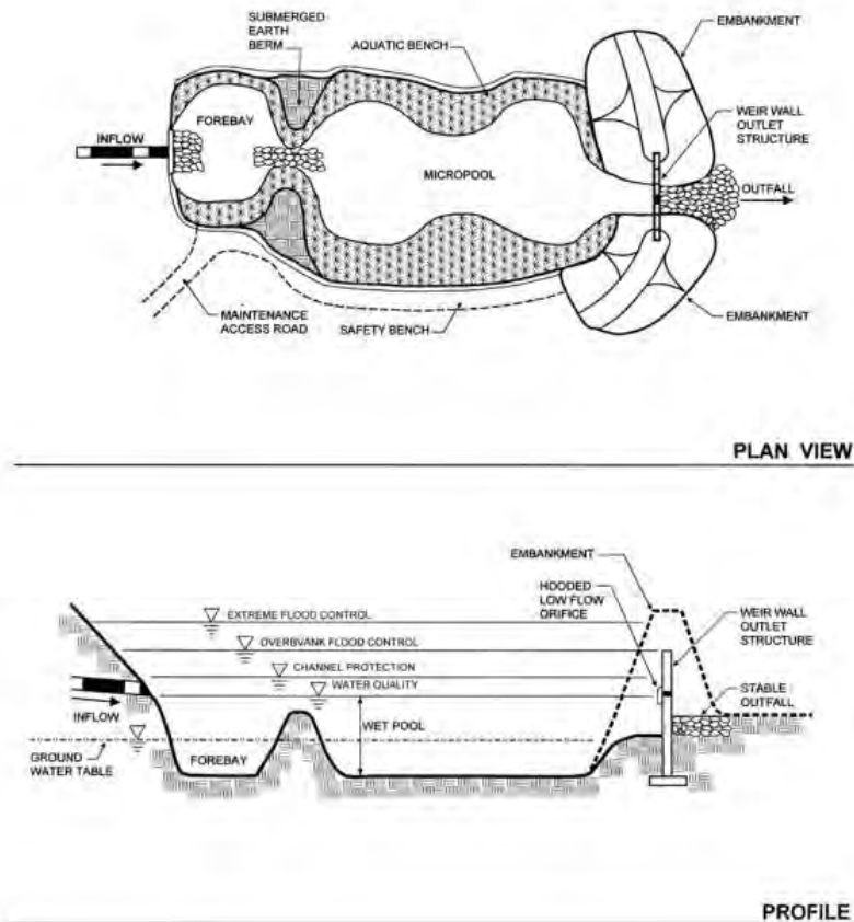
Figure 6.5 Pocket Pond (P-5)
