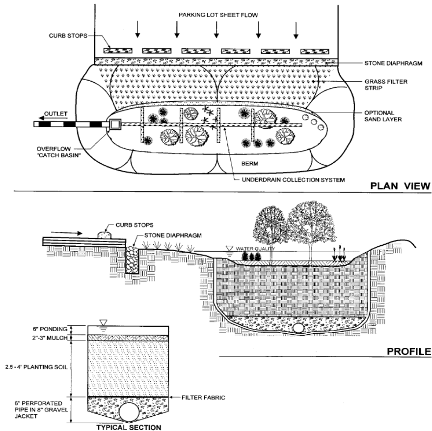
Figure 6.19 Bioretention (F-5)
