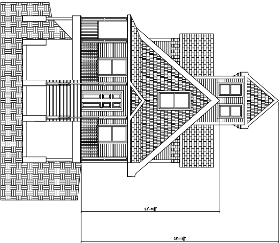
FRONT ELEVATION
