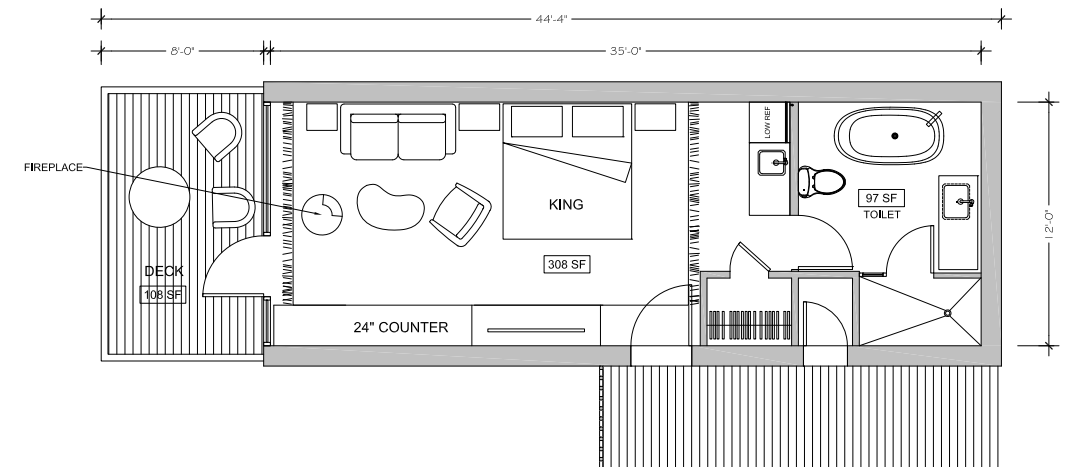
OPTION A - MODULAR INTERIOR SF: 525 GROSS AREA SF: 610
