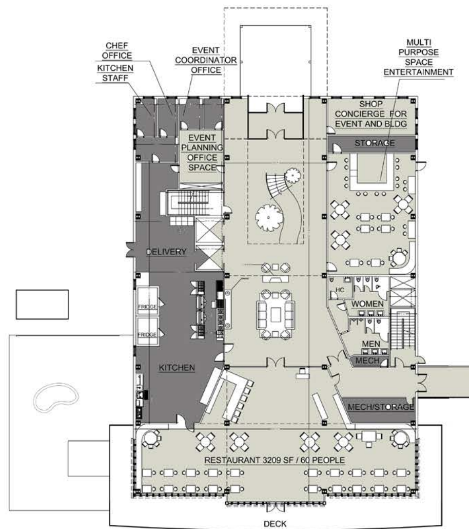
GROUND PLAN
