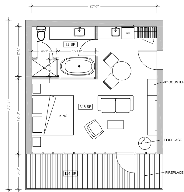
OPTION B - REG. 1 BED INTERIOR SF: 526 GROSS AREA SF: 596
