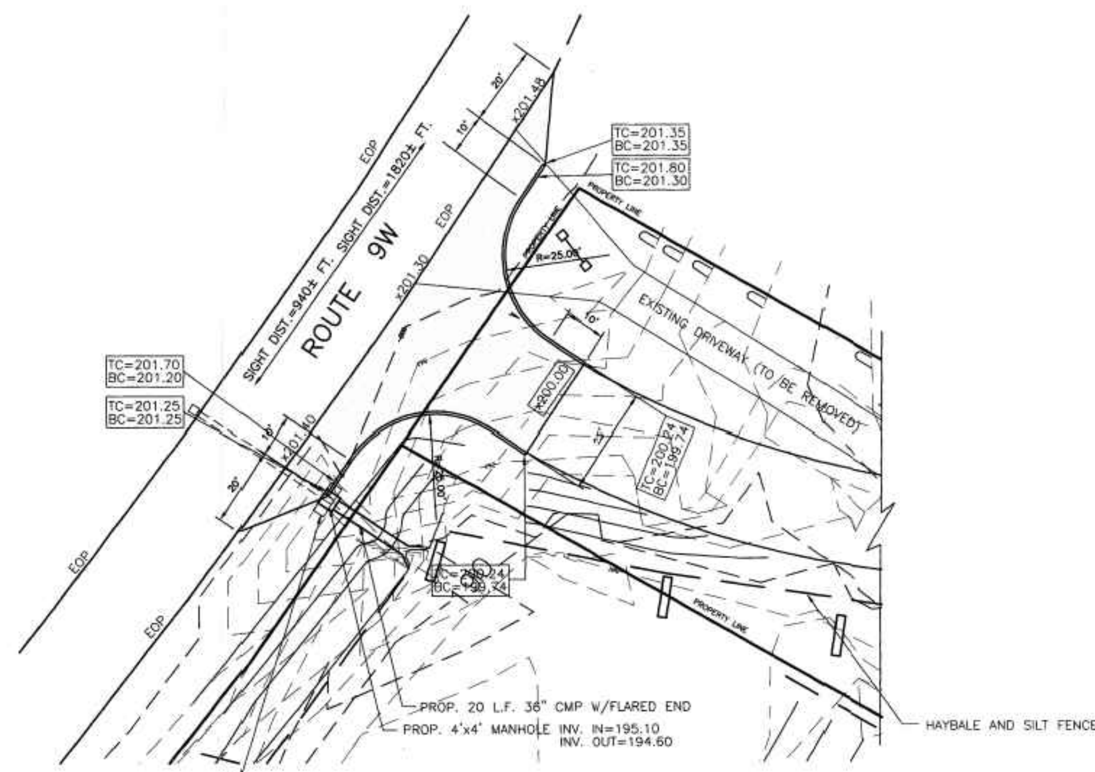
CONTRACTOR TO REMOVE HEADWALL AND TO EXPOSE 2'x2' CONCRETE BOX CULVERT FIELD VERIFY CONCRETE BOX CULVERT SIZE AND INVERT PRIOR TO MANHOLE FABRICATION
